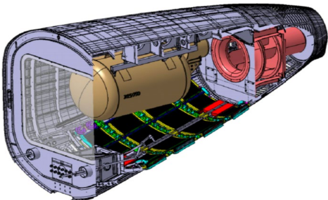
Simulation ILA-Berlin Fuel Cell Tailcone
